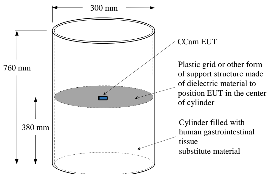
Figure B.1: Human torso simulator fixture (depicted not to scale)
