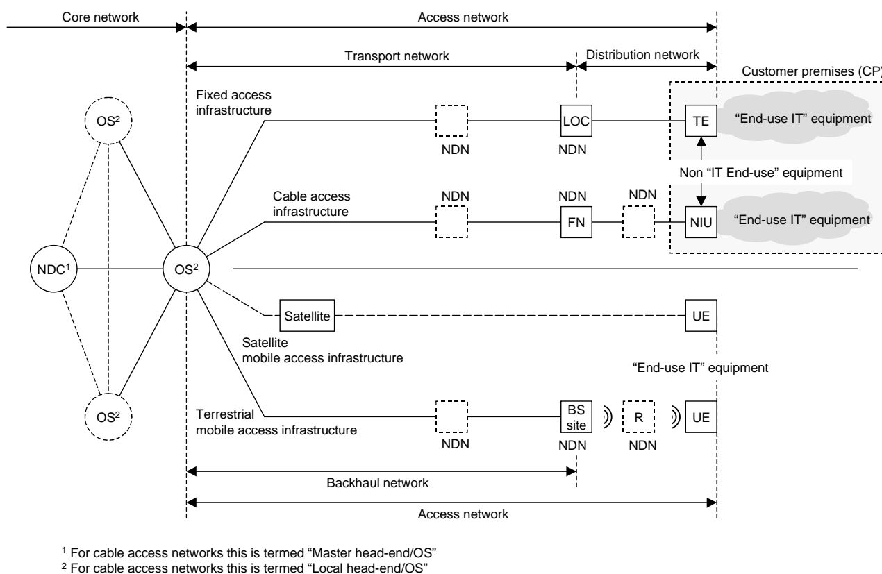
Figure 1: Updated schematic of fixed and mobile access networks
