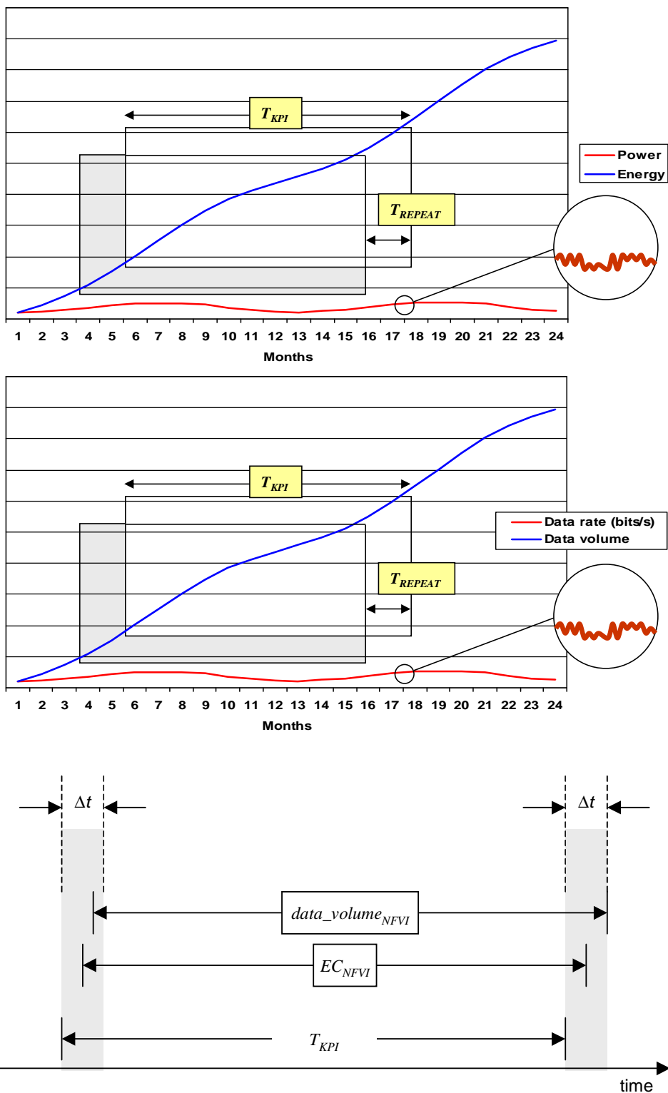
Figure 3: Schematic showing application of T_{KPI} , T_{REPEAT} and \Delta t
