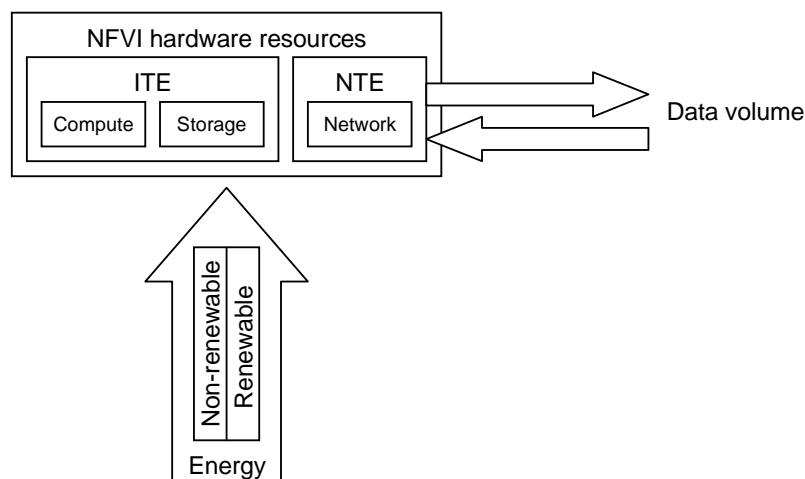
Figure 2: Schematic of KPI_{EE-transfer}
