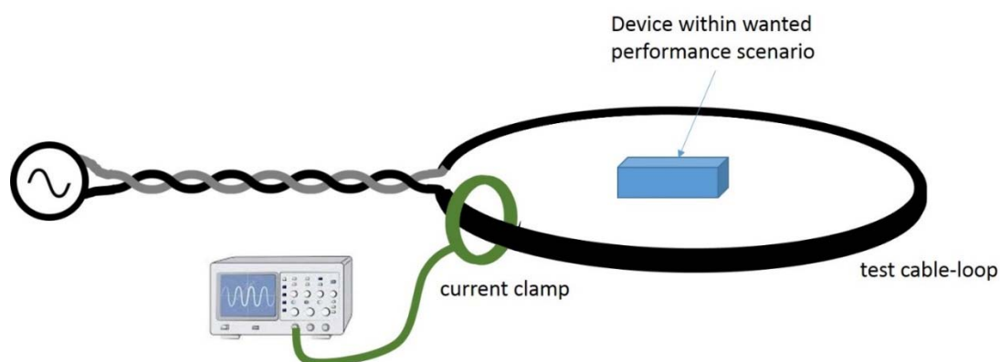
Figure 6: Schematic test set-up for the RX-blocking test
