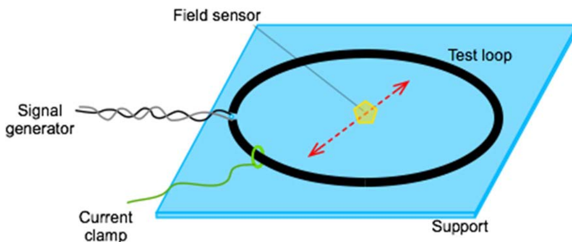
Figure B.3: Test-loop magnetic field verification
