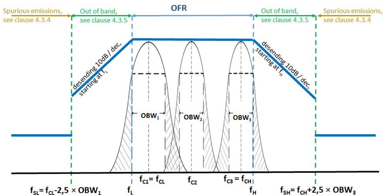
Figure 4: Out of band and spurious domain of a multi-frequency system
