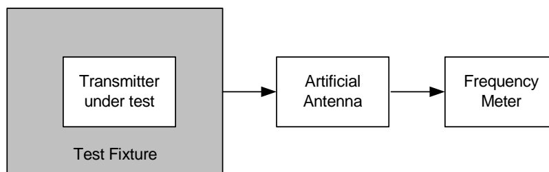
Figure 2: Measurement arrangement
