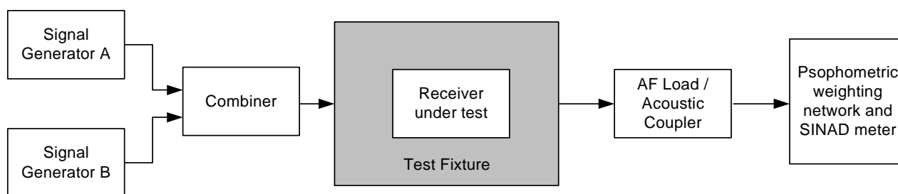
Figure 17: Measurement arrangement
