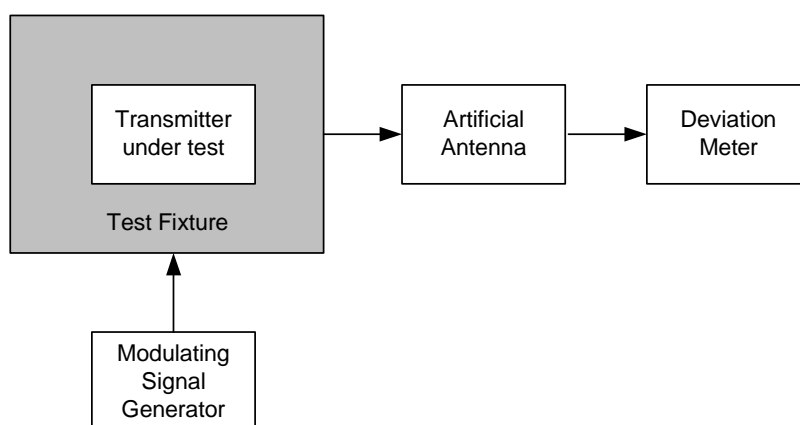
Figure 6: Measurement arrangement
