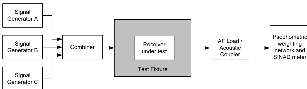
Figure 19: Measurement arrangement
