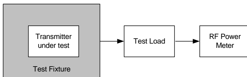
Figure 5: Measurement arrangement
