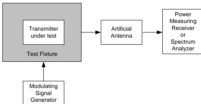
Figure 8: Measurement arrangement
