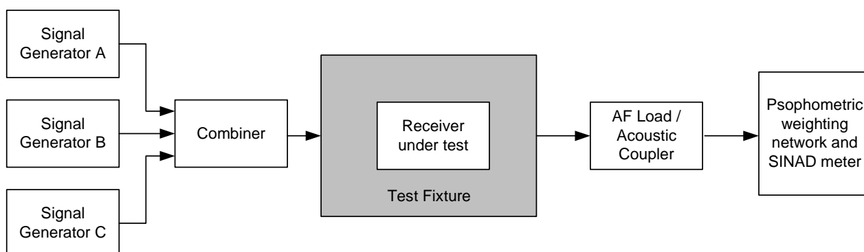
Figure 19: Measurement arrangement
