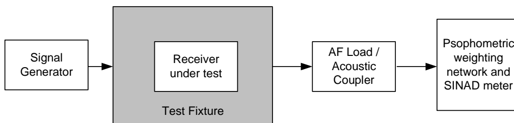
Figure 13: Measurement arrangement
