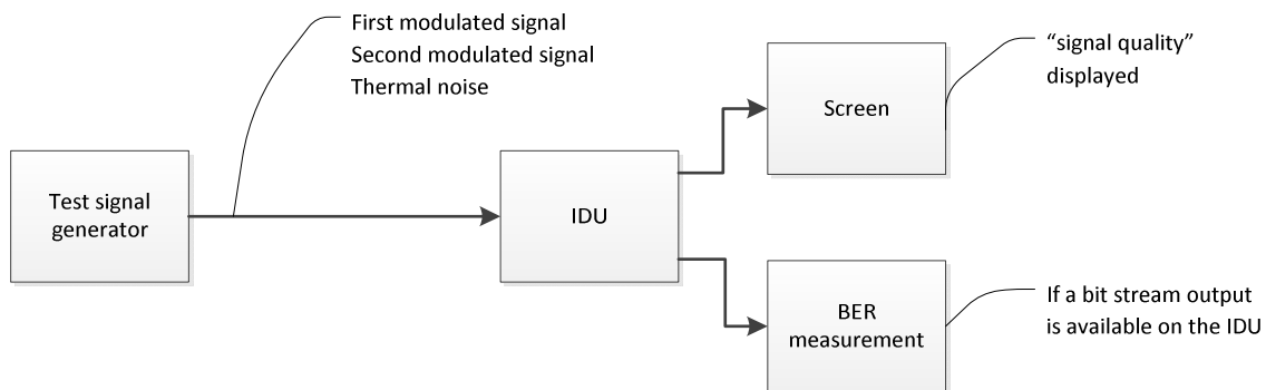
Figure 2: Test set-up for adjacent signal selectivity with generator capable of two modulated signals
