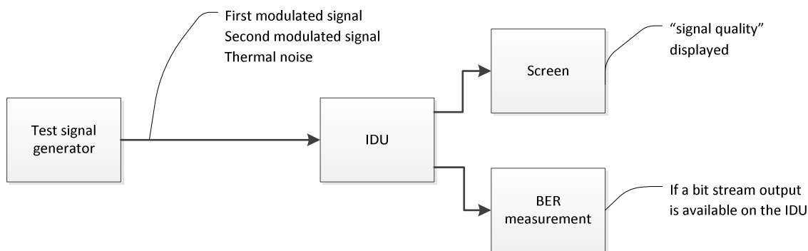
Figure 2: Test set-up for adjacent signal selectivity with generator capable of two modulated signals
