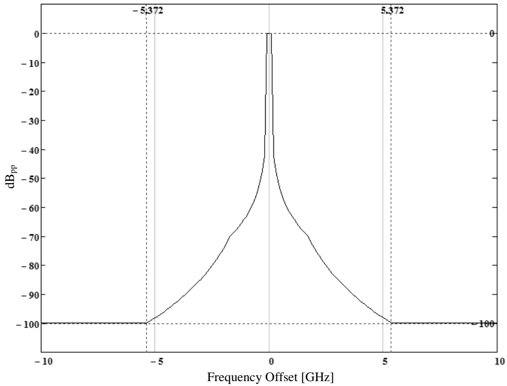
Figure 4: Calculated emission mask for typical pulse duration of t = 50 ns and rise time of t_r = 10 ns (single carrier frequency)
