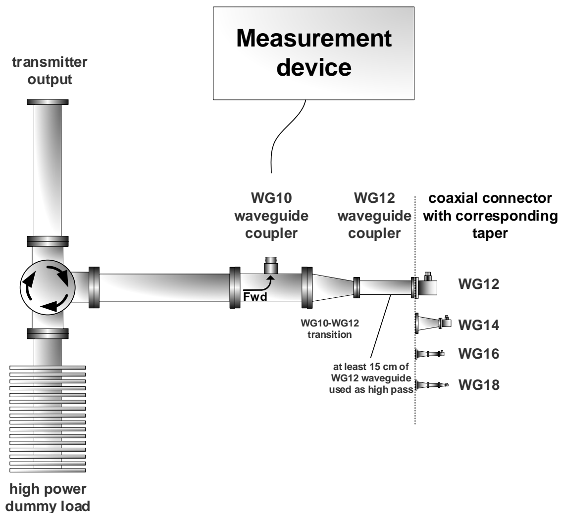
Figure D.1: Indirect method for spurious emission measurement
