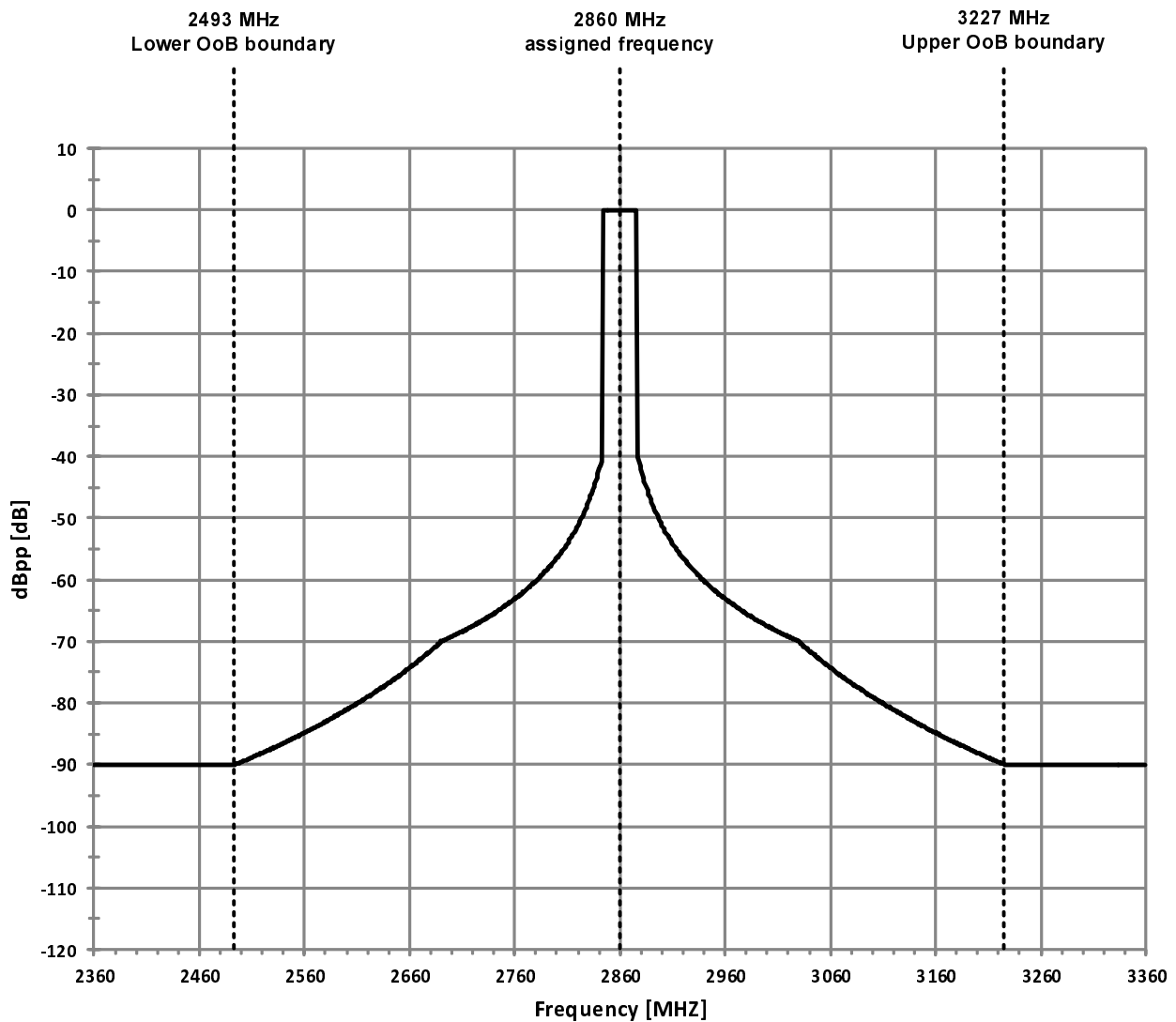
Figure 7: Calculated emissions mask for pulse duration t = 500 ns and rise time t_r = 100 ns at centre frequency of 2 860 MHz
