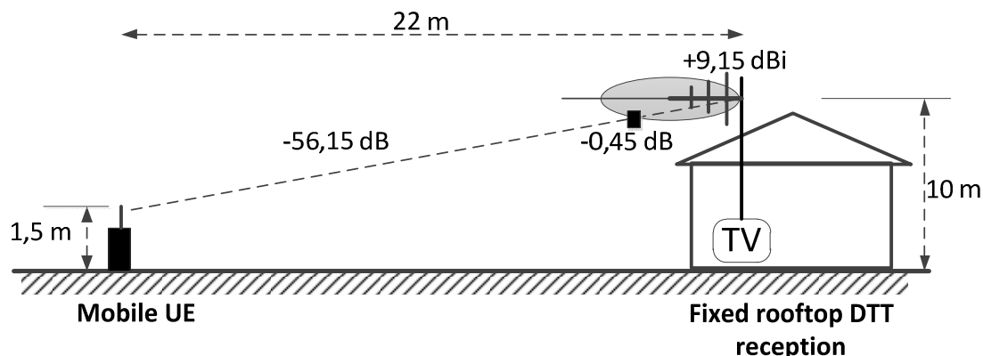
Figure B.8: Reference model for coupling gain
