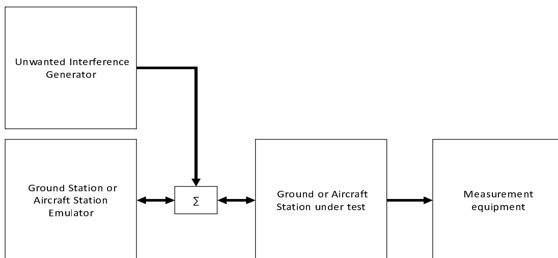
Figure B.3: Measurement system for receiver blocking
