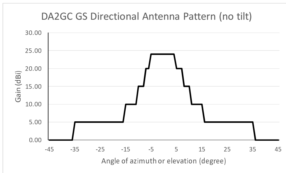
Figure 3: Antenna Radiation Pattern Envelope - Directional - Ground Station
