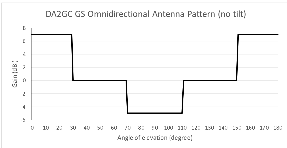
Figure 4: Antenna Radiation Pattern Envelope - Omni - Ground Station
