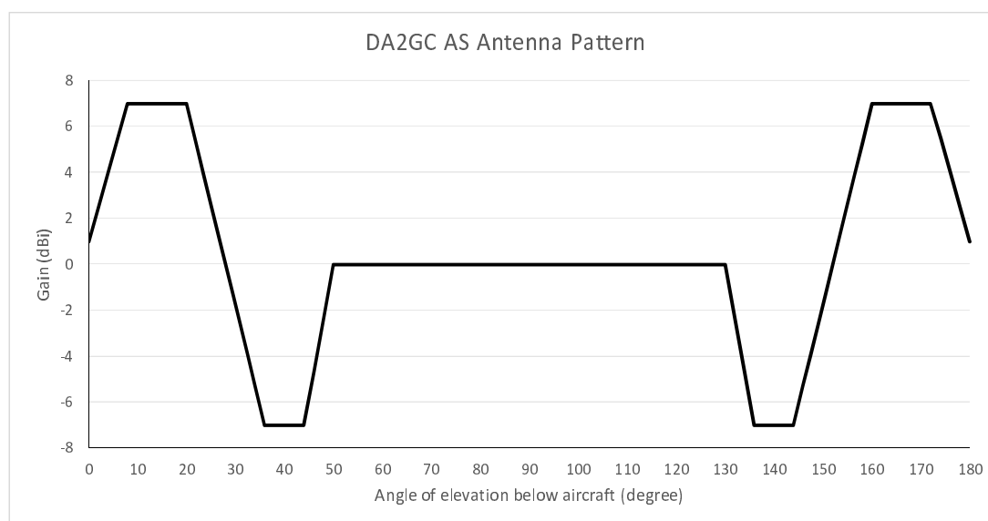
Figure 1: Antenna Radiation Pattern Envelope - Aircraft Station
