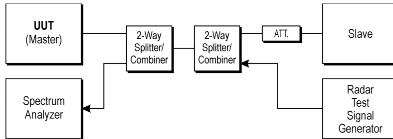
Figure 3: Set-up A
