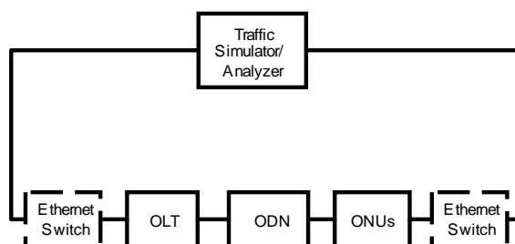
Figure 4: Test Setup for power measurement for OLT
