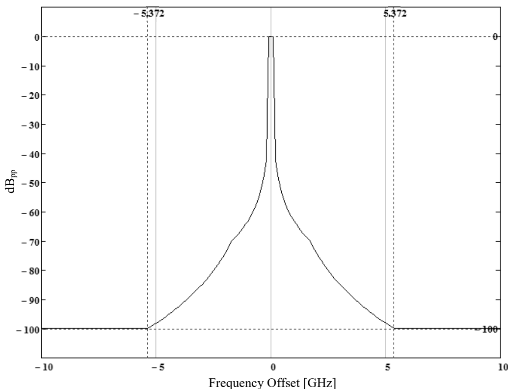
Figure 4: Calculated emission mask for typical pulse duration of t = 50 ns and rise time of t_r = 10 ns
