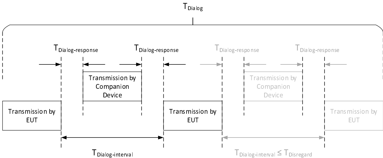
Figure 7: SCS dialog timing constraints
