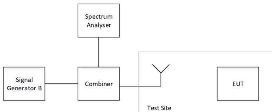
Figure 10: Radiated clear channel assessment threshold measurement arrangement
