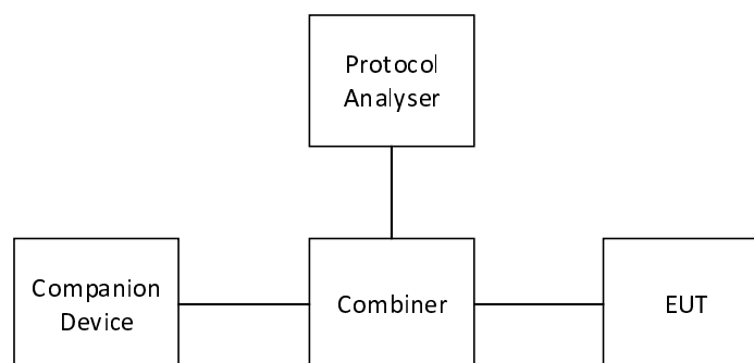
Figure 13: SCS transmissions measurement arrangement
