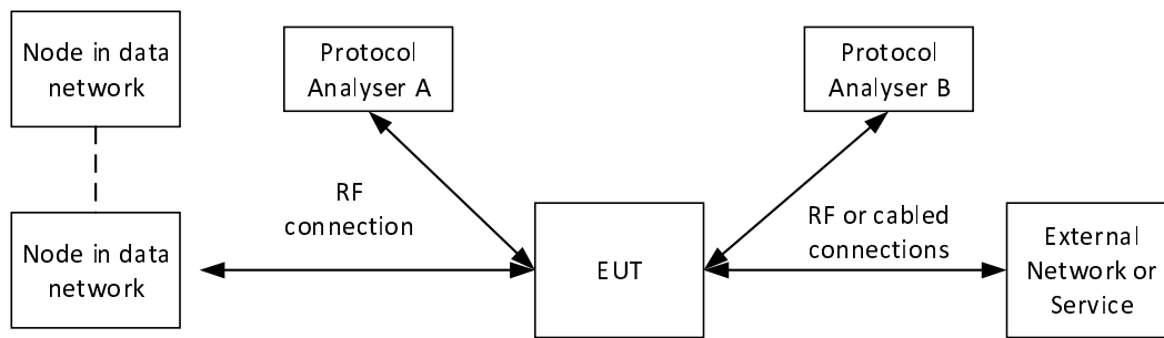
Figure 14: Network access point analyser arrangement
