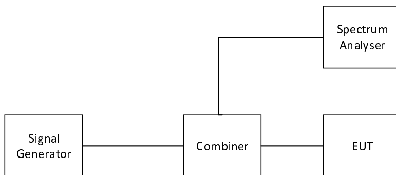
Figure 9: Conducted clear channel assessment threshold measurement arrangement
