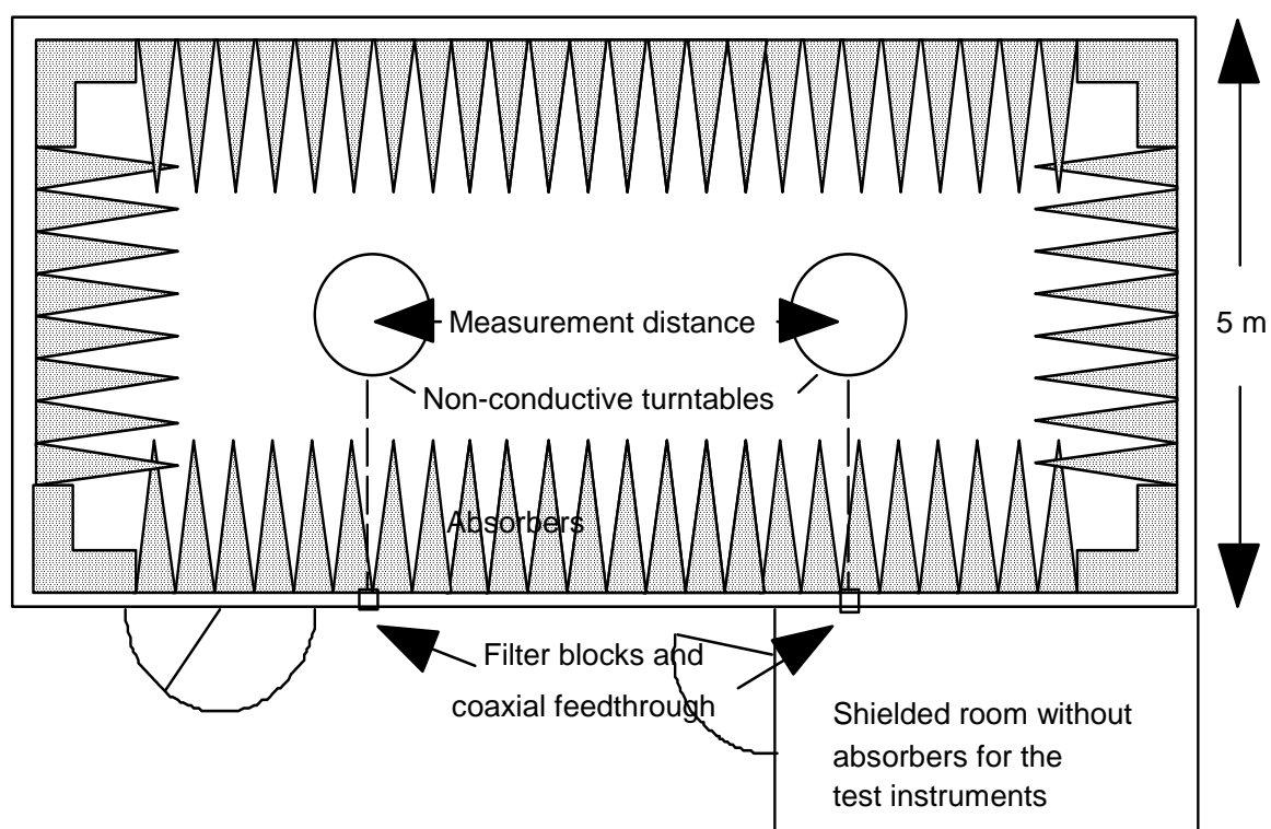
Ground plan
