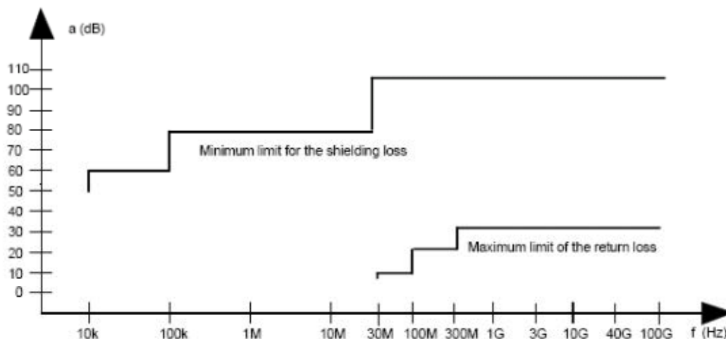
Figure B.4: Specification for shielding and reflections
