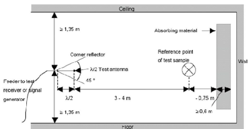
Figure B.2: Indoor test site
