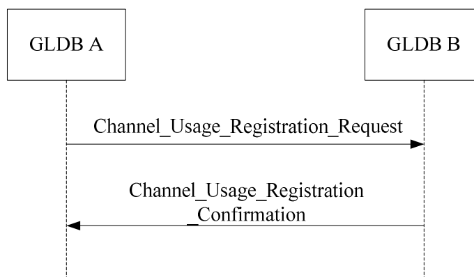
Figure 6.7: CRS channel usage registration procedure
