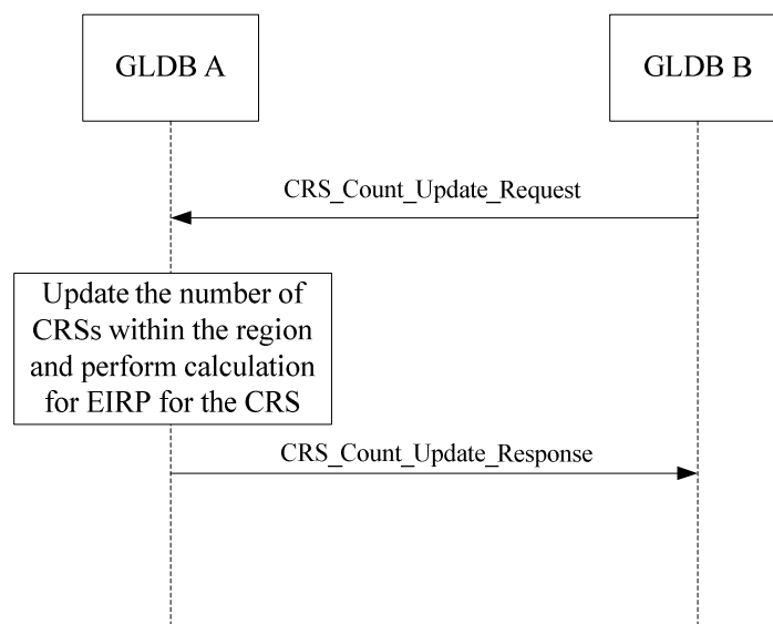
Figure 6.9: CRS number update procedure
