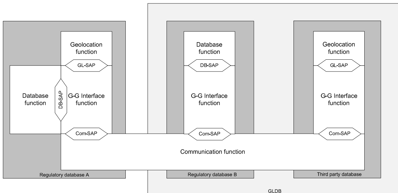
Figure A.2: Implementation example of third party database
