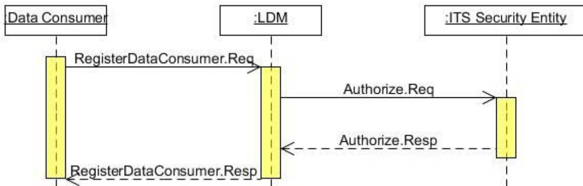
Figure 11: RegisterDataConsumer message sequence
