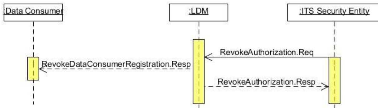
Figure 13: RevokeDataConsumerRegistration message sequence
