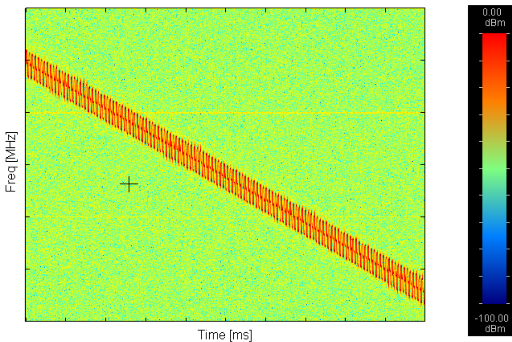
Figure 6: Example of spectrogram measurement result
