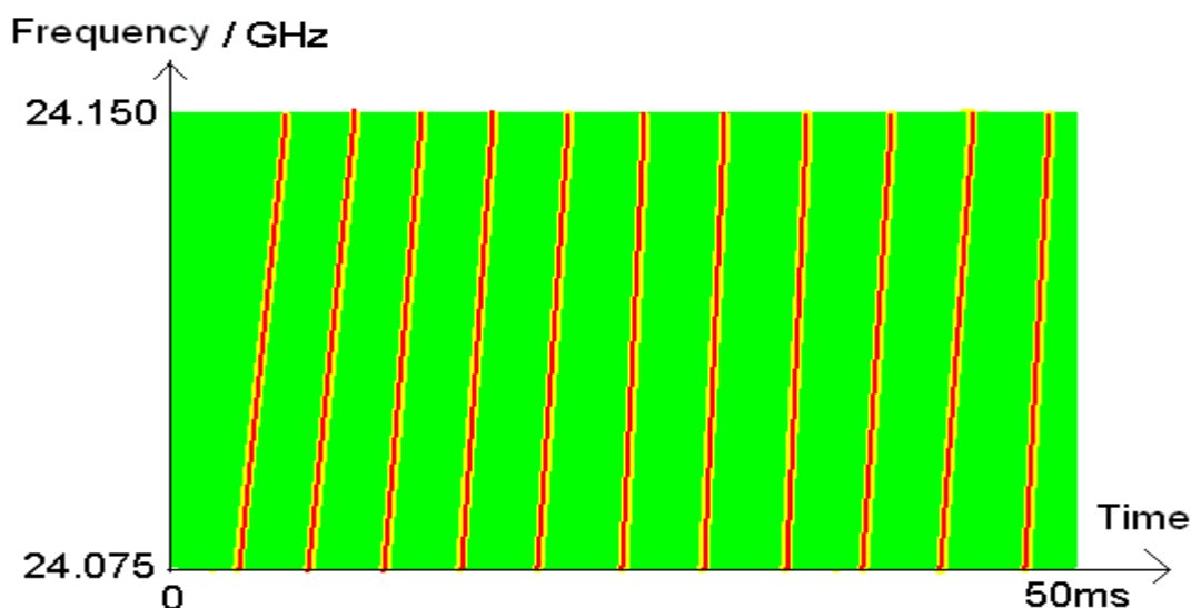
Figure 11: Example of a spectrogram of a signal analysis measurement for a fast modulation signal
