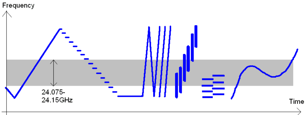
Figure 7: Examples of NB SRR transmit frequency signals versus time
