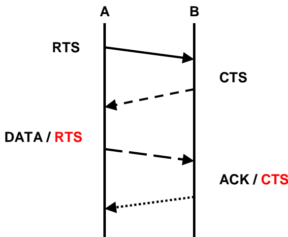
Figure 4.6: Linked transmissions
