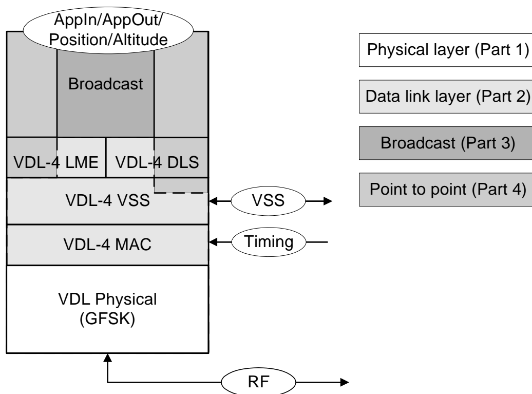
Figure 4.3: Structure of VDL Mode 4 mobile station specifications
