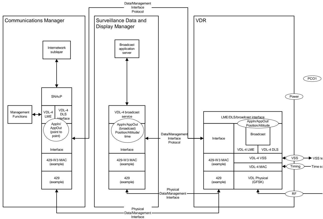
Figure 4.2: Possible VDL Mode 4 aircraft architecture
