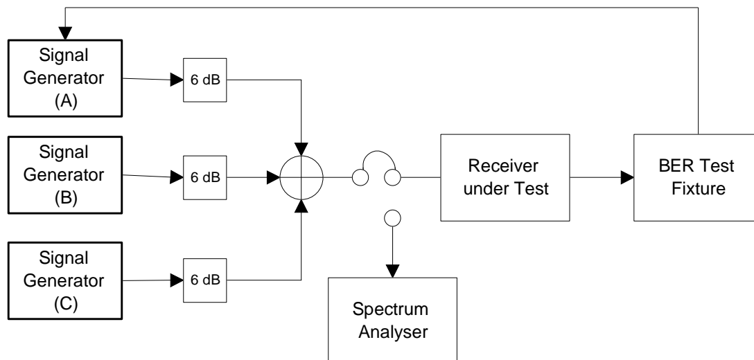
Figure 9.2: Intermodulation measurement
