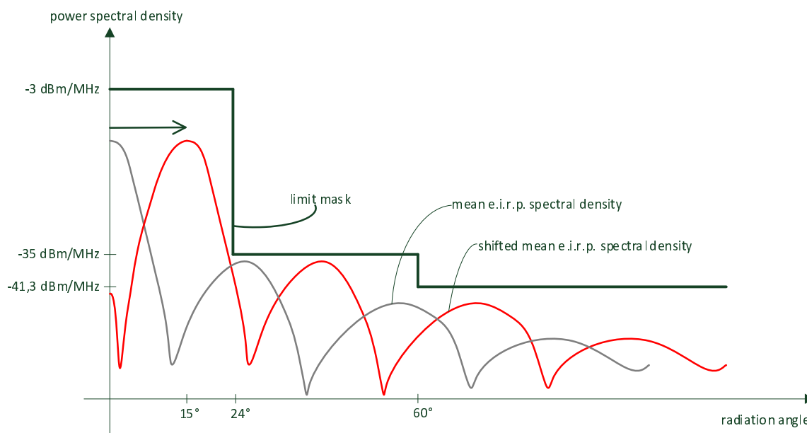
Figure 5: Limit mask for TiltLPR1 devices with exemplary EUT radiation pattern and the shifted curve
