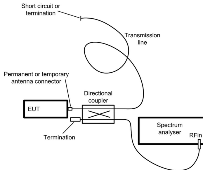
Figure 8: Measurement setup for the equivalent conducted APC conformance test method
