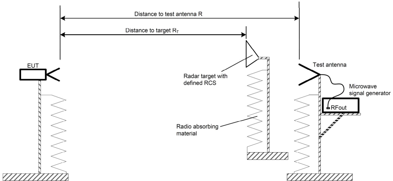
Figure 7: Radiated test setup providing a defined echo signal and an interferer signal to the EUT
