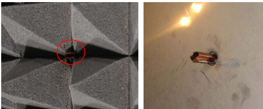
Figure 3: Left: Horn antenna fitted in pyramidal absorbers; Right: Horn antenna protruding the centre of the metal plate
