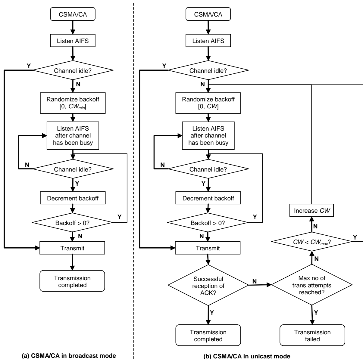
Figure B.2: A simplified drawing of the channel access procedure in IEEE 802.11-2012 [3] in broadcast and unicast mode
