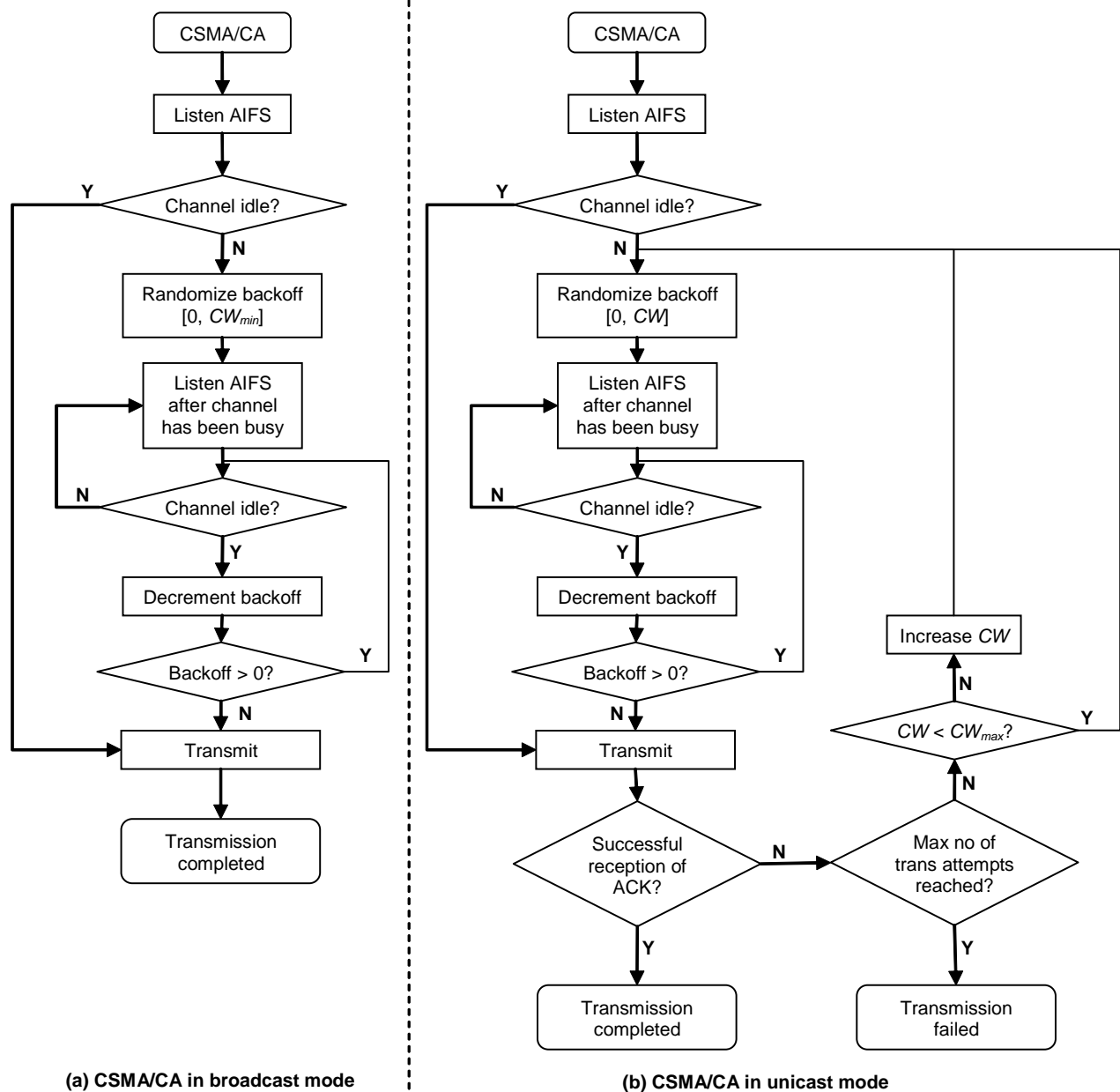
Figure B.2: A simplified drawing of the channel access procedure in IEEE 802.11-2012 in broadcast and unicast mode
