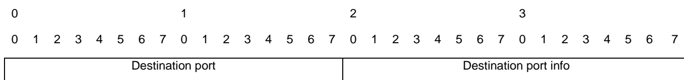
Figure 5: BTP-B header format
