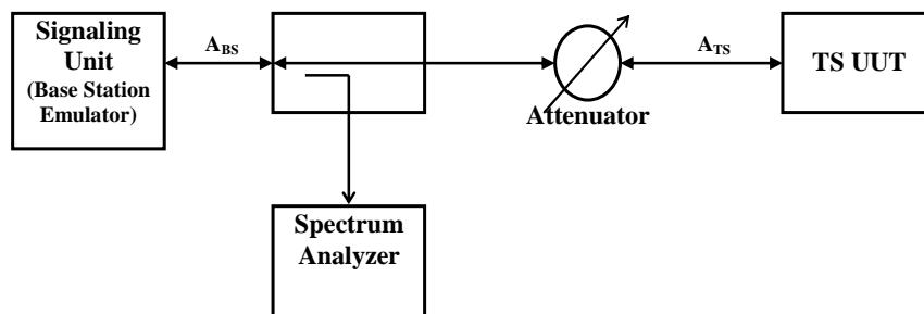
Figure 1: Test setup for spectral mask emission testing
