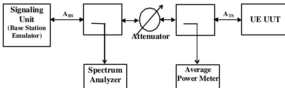
Figure 4: Test setup for transmitter output power and transmit power control
