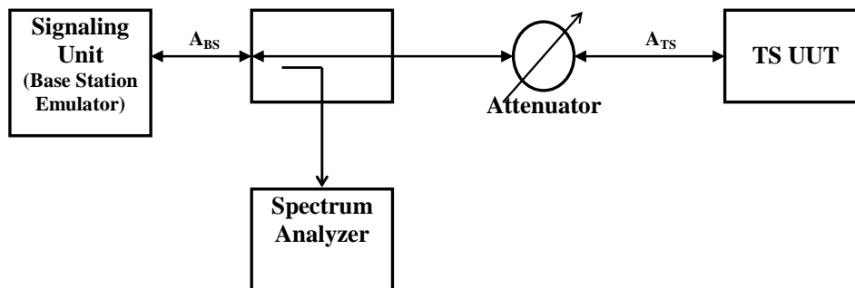
Figure 5: Test setup for receiver spurious emission testing
