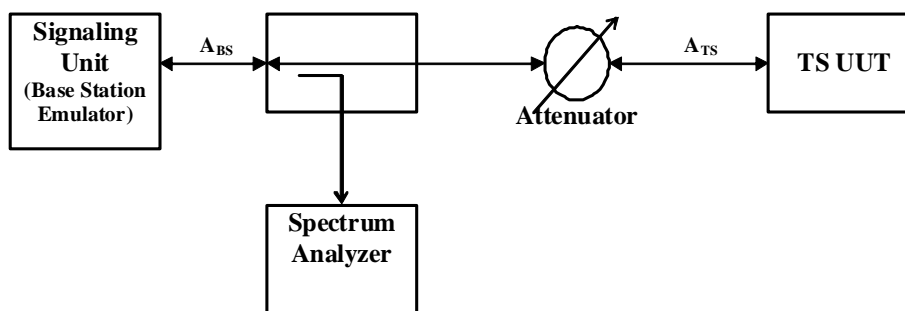
Figure 3: Test Setup for transmitter spurious emission testing
