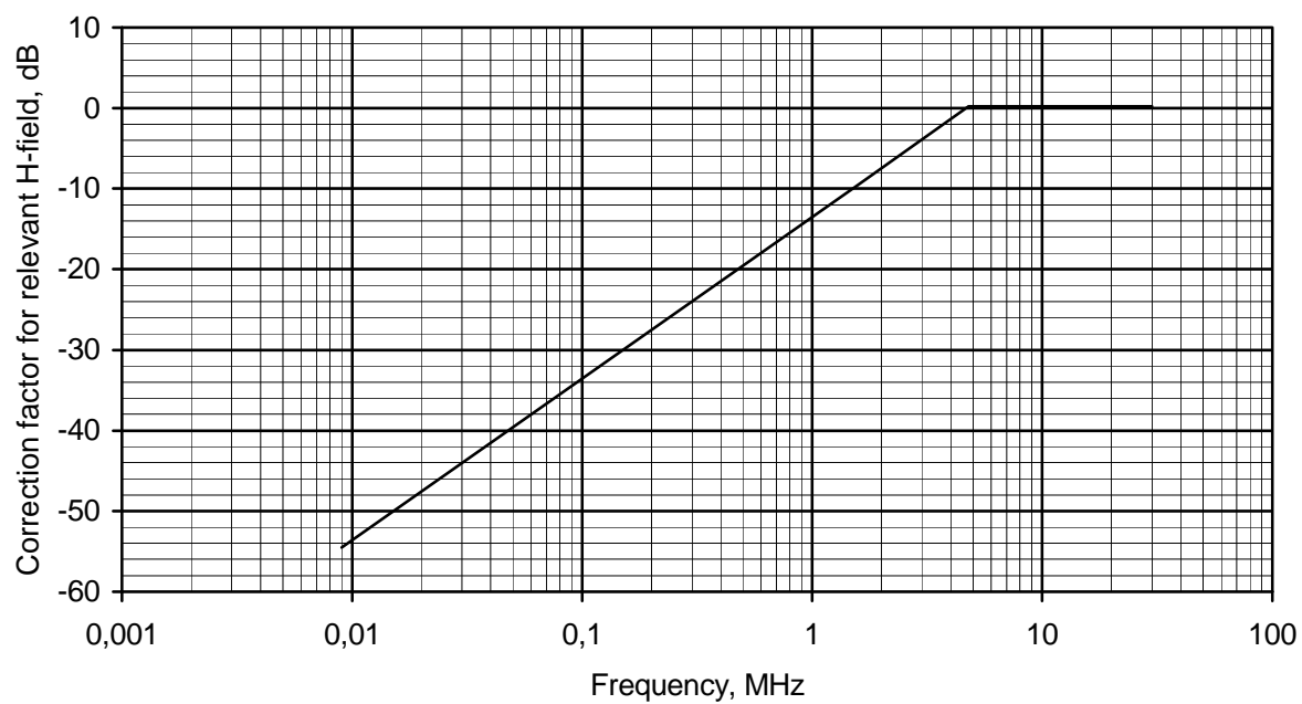
Figure E.1: Conversion factor C30 versus frequency
