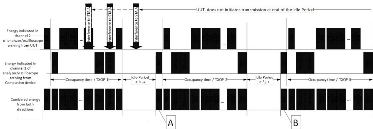
Figure 3: Channel 1/2 chronogram
