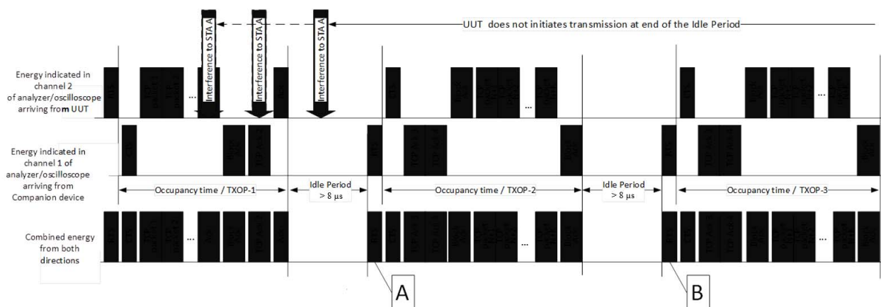
Figure 3: Channel 1 / 2 chronogram
