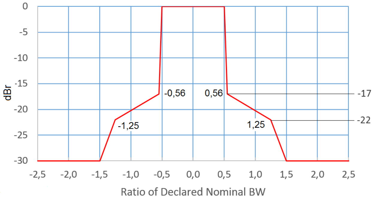
Figure 1: Transmit Mask
