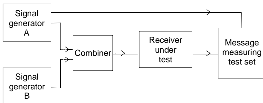
Figure 10: Measurement arrangement
