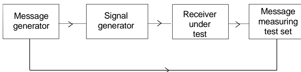
Figure 6: Measurement arrangement
