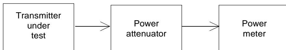
Figure 1: Measurement arrangement
