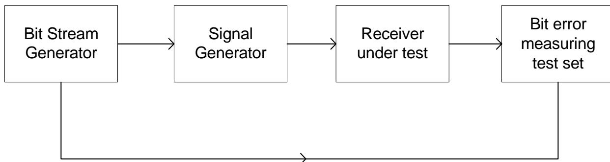
Figure 5: Measurement arrangement
