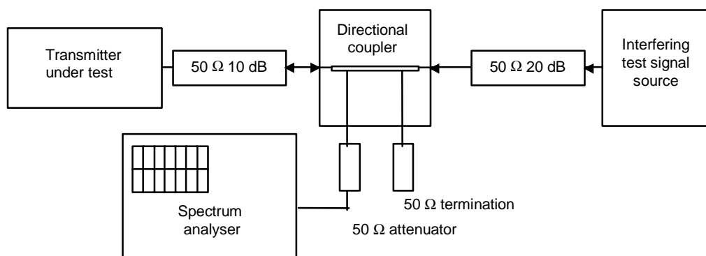
Figure 3: Measurement arrangement
