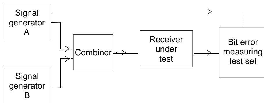
Figure 7: Measurement arrangement
