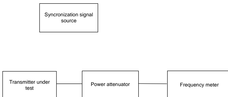
Figure 4: Measurement arrangement
