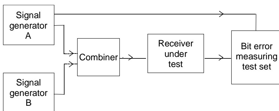
Figure 9: Measurement arrangement
