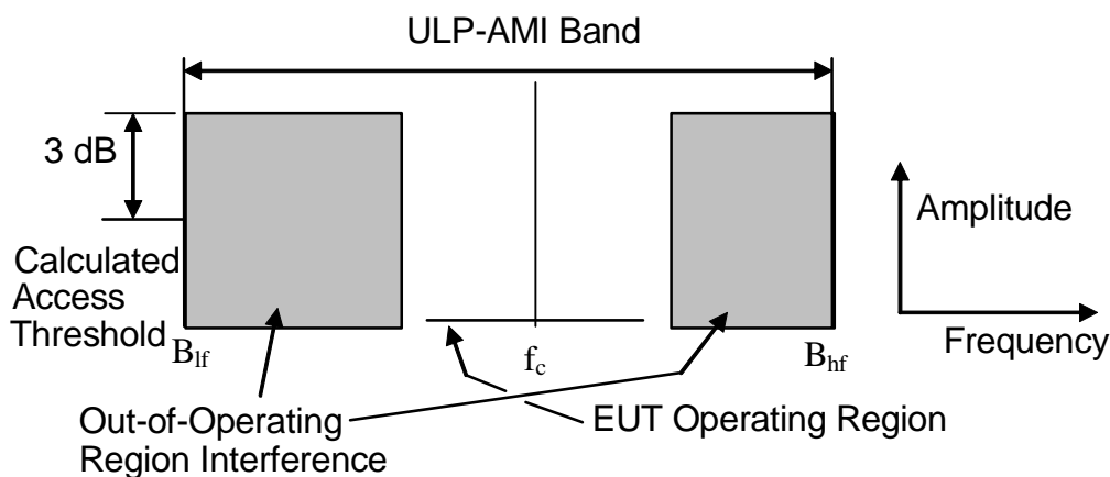
Figure 3: Spectrum mask for test of clause 5.3.8.1.2.1
