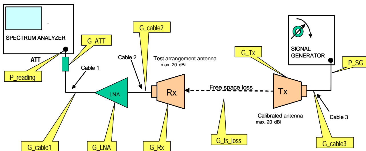
Figure A.3: Calibration set-up configuration
