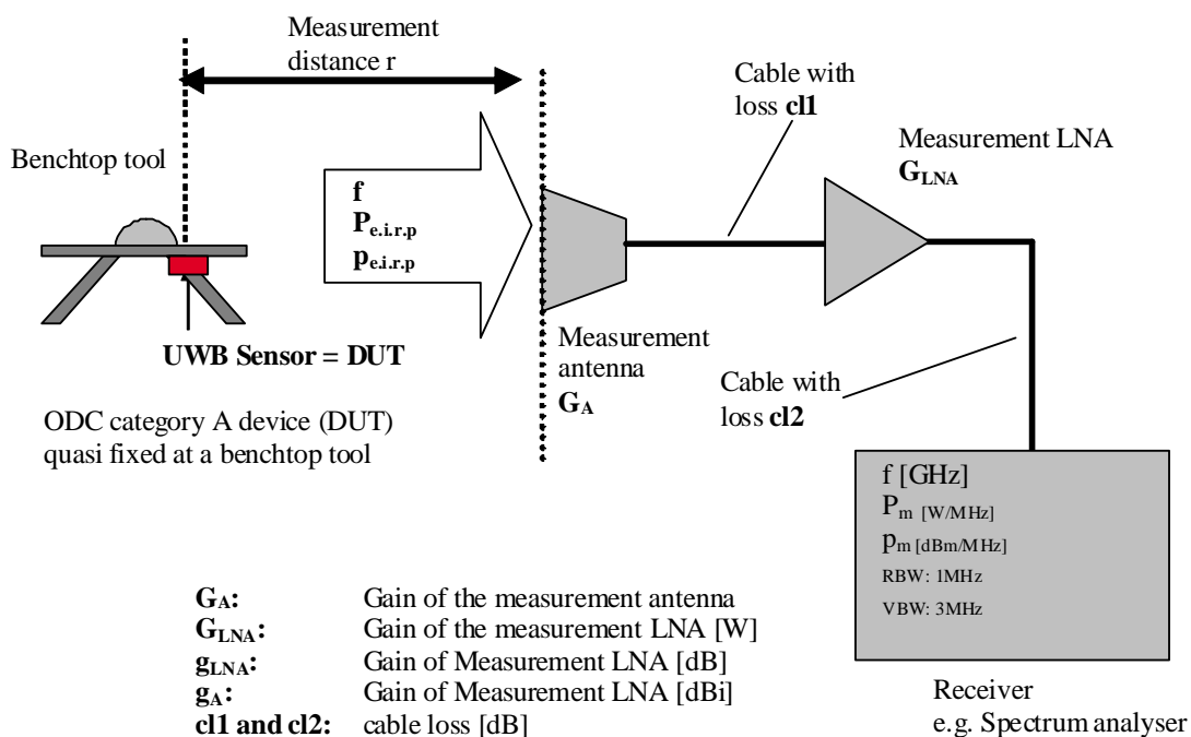
Figure 7a: Test set-up for e.i.r.p measurement for Category A equipment
