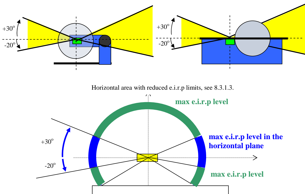
Figure 7b: Spatial requirements for the test set-up
