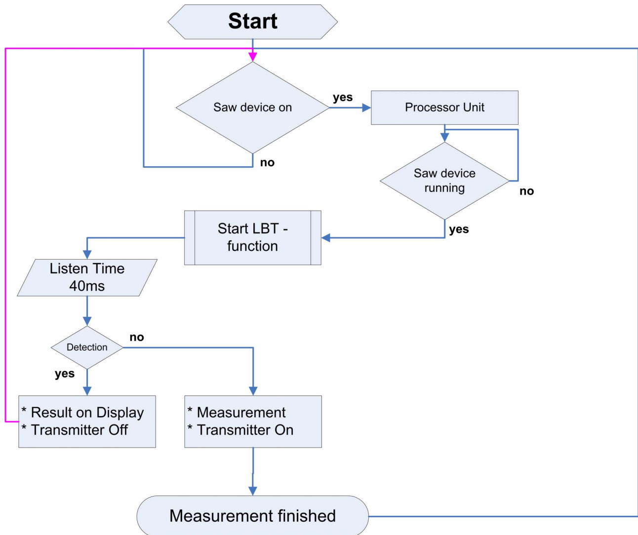
Figure 9: Flow diagram of LBT mechanism for Category A
