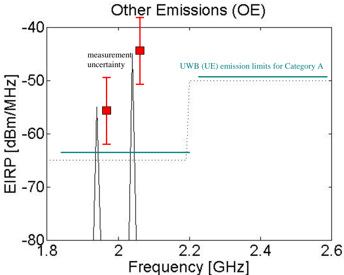
Figure 4: Example for a OE measurement in the frequency range 1,8 GHz to 2,6 GHz
