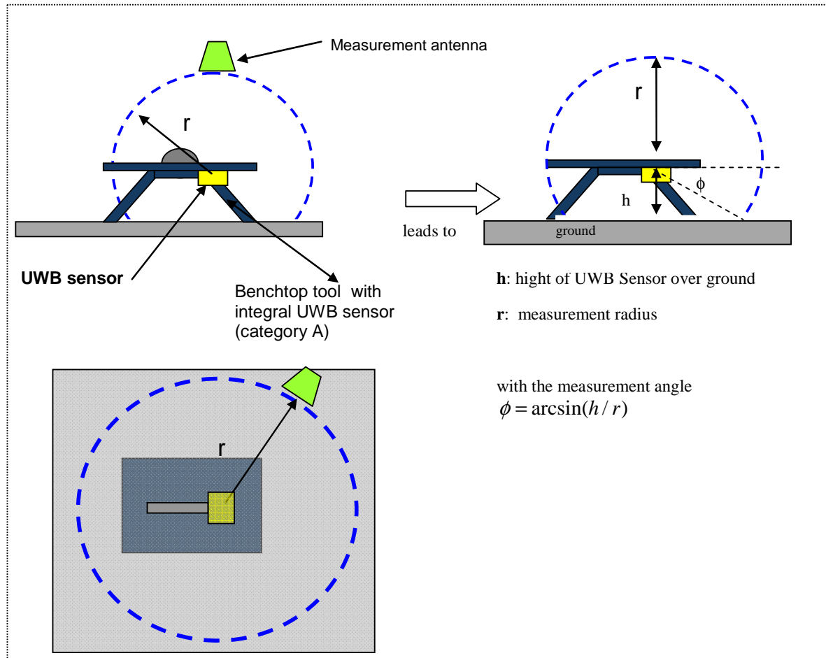
Figure 5: Measurement arrangement for all emission measurements (TE, UE, OE, UE-TP) for Category A equipment
