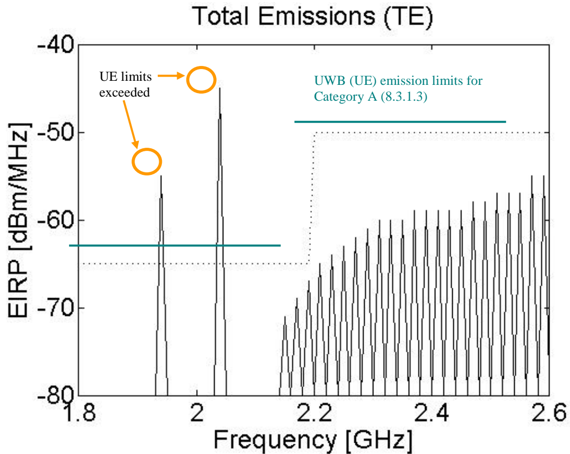
Figure 3: Example for a TE measurement in the frequency range 1,8 GHz to 2,6 GHz
