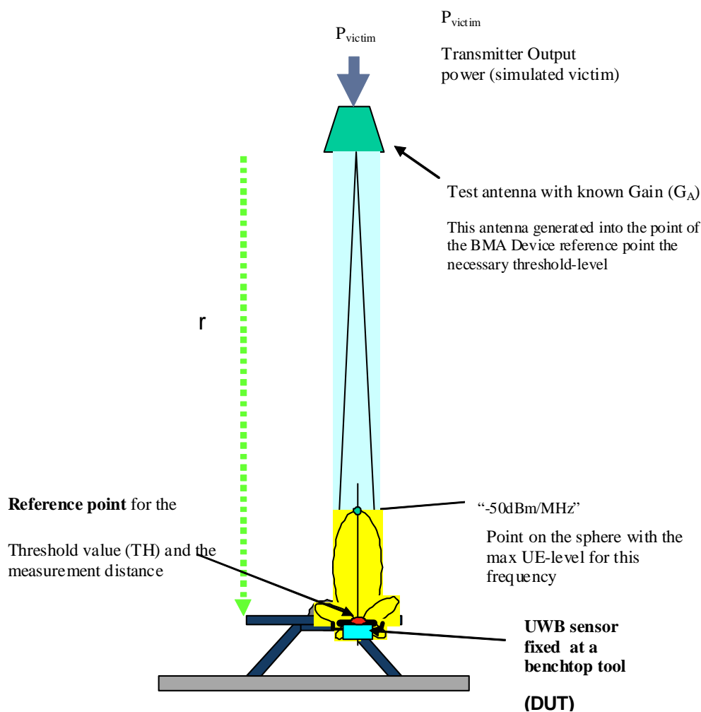
Figure 11: Test set-up for LBT function for category A equipment
