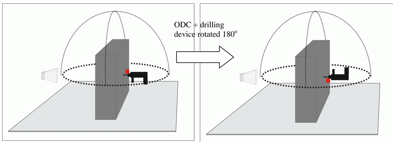
Figure 6: Measurement arrangement for all emission measurements (TE, UE, OE, UE-TP) for Category B equipment
