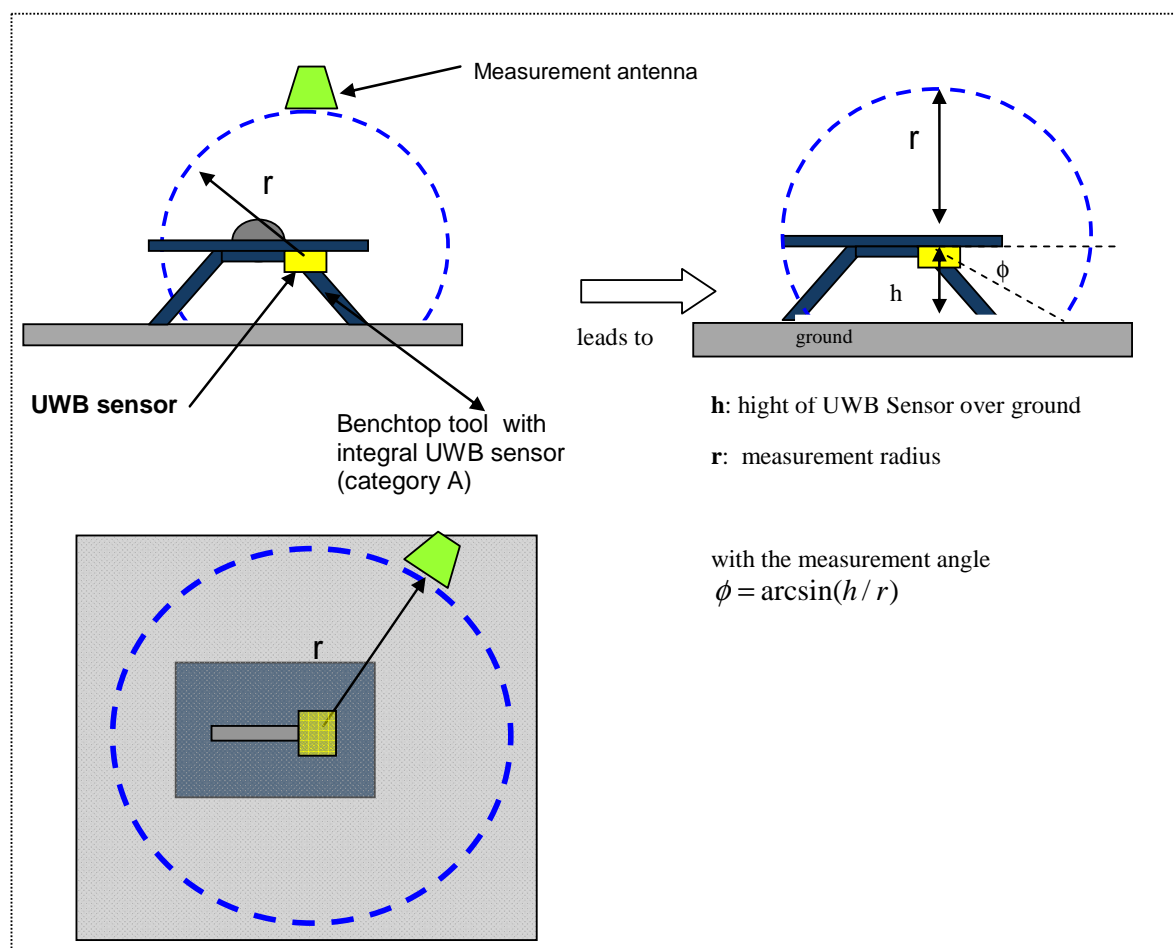
Figure 5: Measurement arrangement for all emission measurements (TE, UE, OE, UE-TP) for Category A equipment
