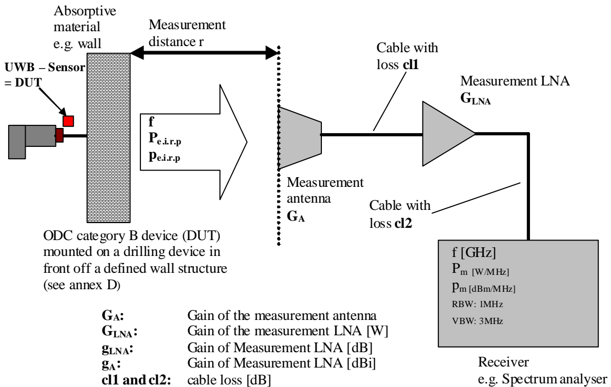
Figure 8a: Test set-up for e.i.r.p measurement for Category B equipment
