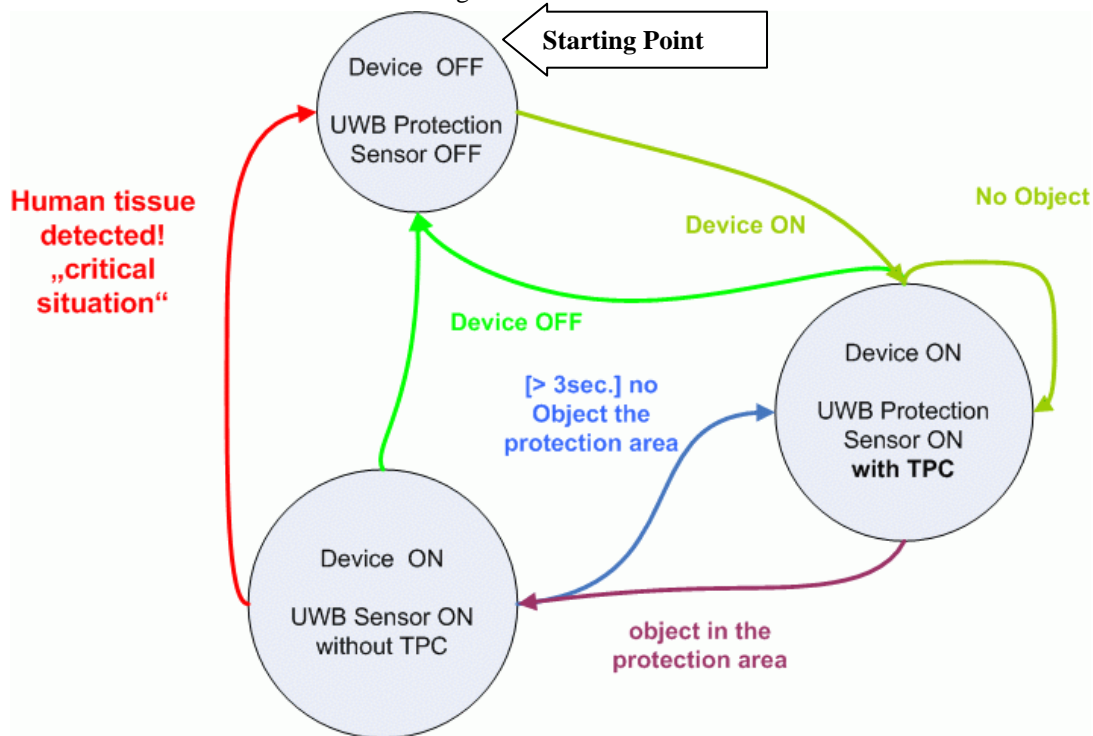
Figure 16: TPC - procedure for category A equipment
