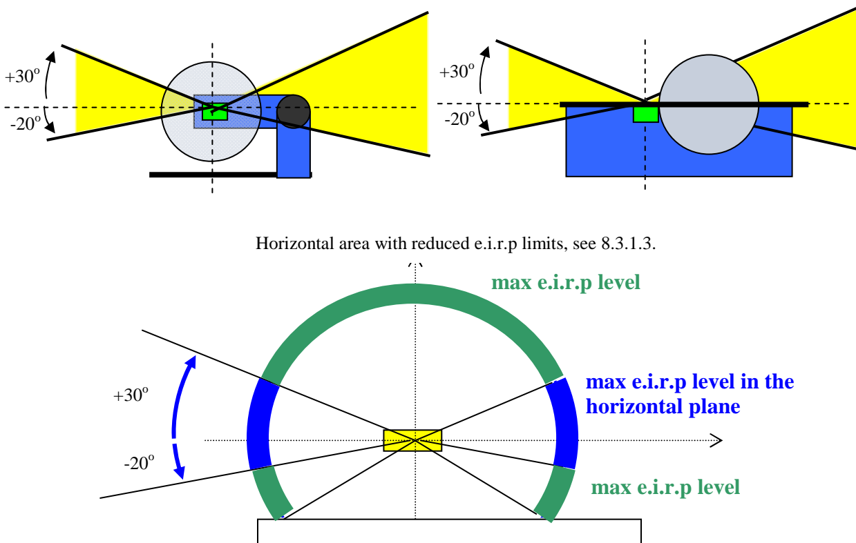
Figure 7a: Test set-up for e.i.r.p measurement for Category A equipment
