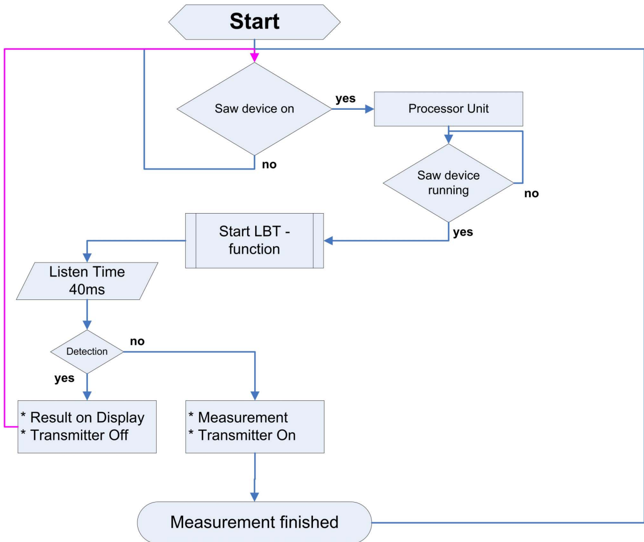
Figure 9: Flow diagram of LBT mechanism for Category A
