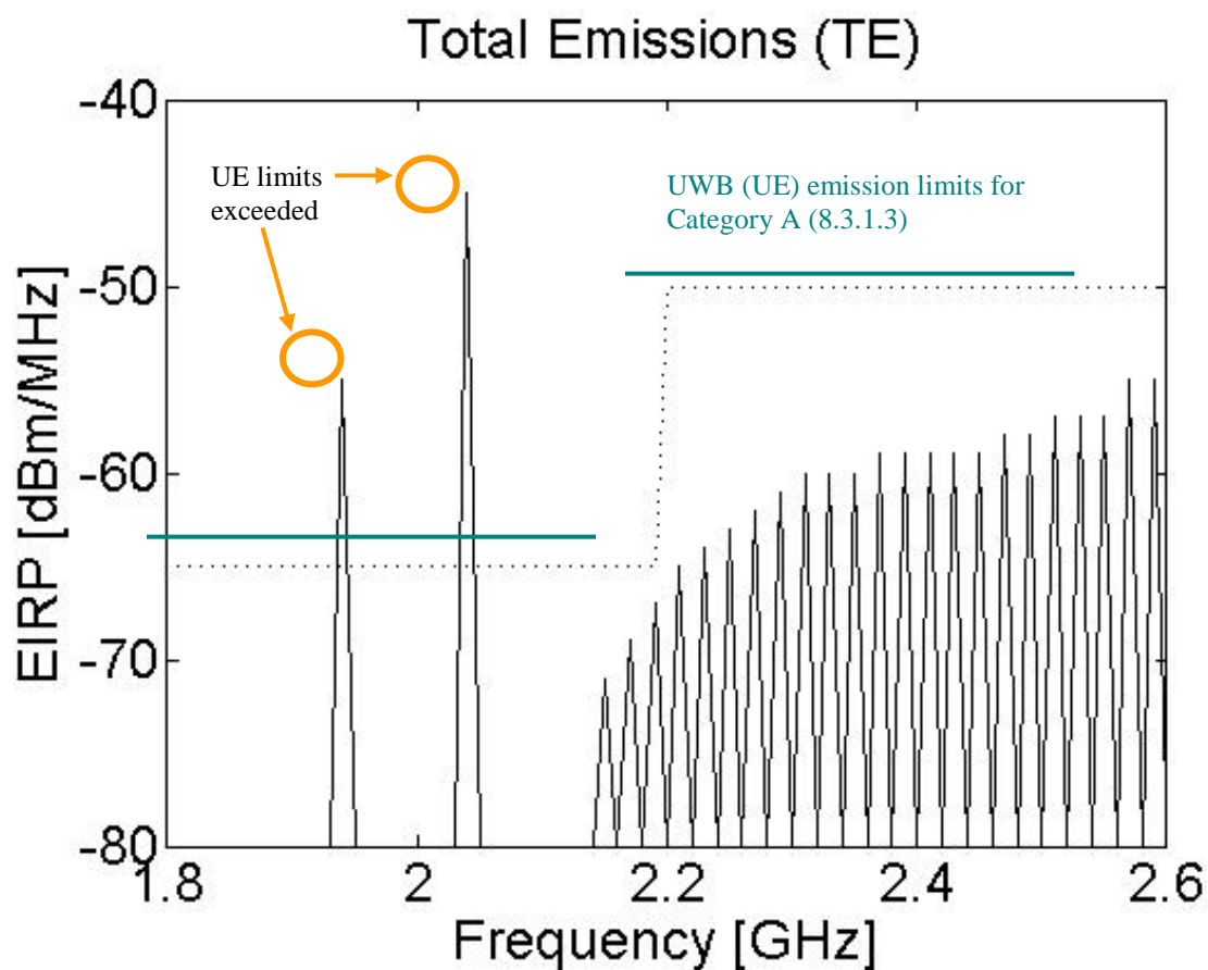
Figure 3: Example for a TE measurement in the frequency range 1,8 to 2,6 GHz
