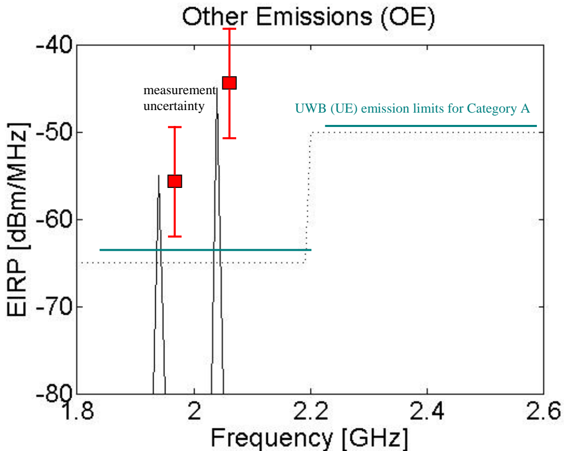
Figure 4: Example for a OE measurement in the frequency range 1,8 to 2,6 GHz
