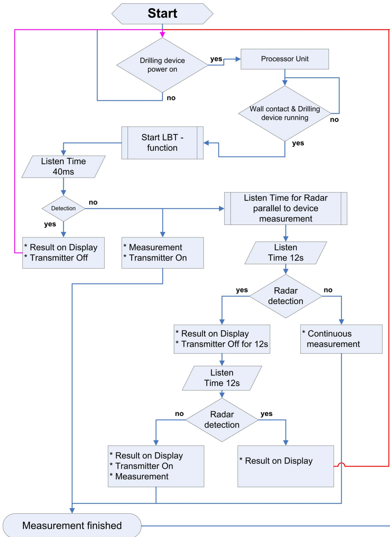
Figure 10: Flow diagram of LBT mechanism for Category B
