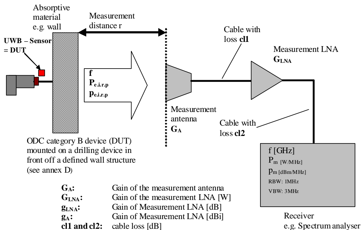
Figure 2: Test set-up for measuring the operating frequency range
