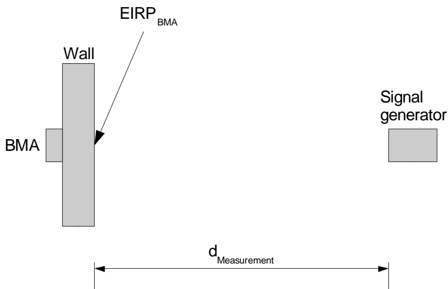
Figure 14: Calculation principle (2)
