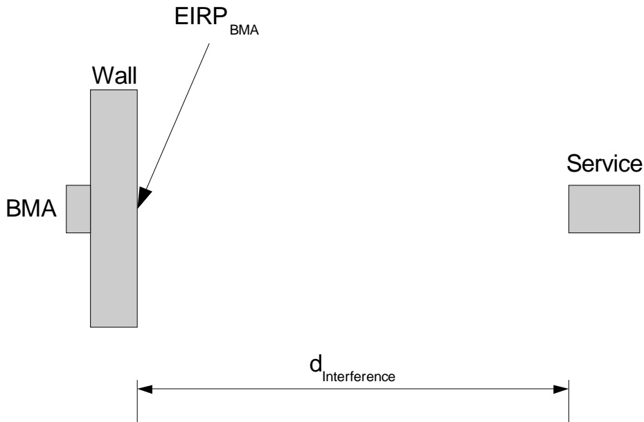
Figure 13: Calculation principle (1)
