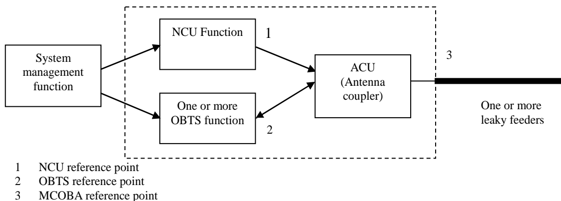
Figure C.1-2: System description for a combined NCU and OBTS signal output
