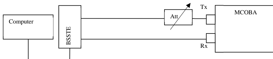
Figure 5.2.3.1.2-1: Test setup
