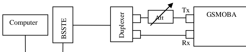
Figure 3: Measurement setup
