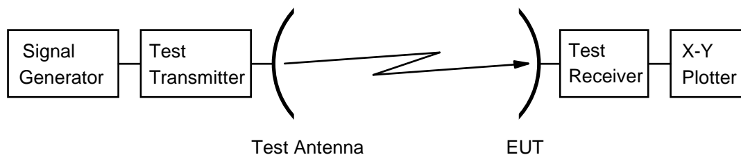
Figure 3: Test arrangement - antenna receive pattern measurement
