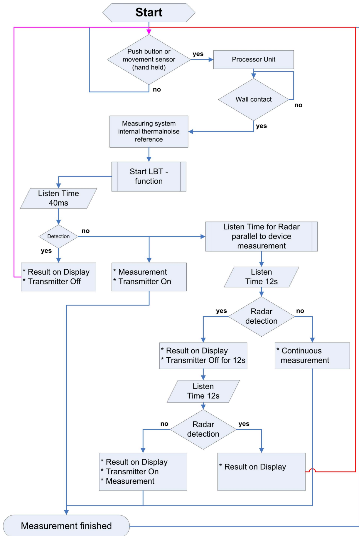
Figure 5: Flow diagram of LBT mechanism
