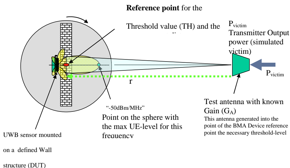
Figure 6: Test set-up for LBT function
