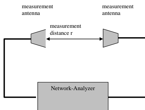
Figure D.1: Calibration setup
