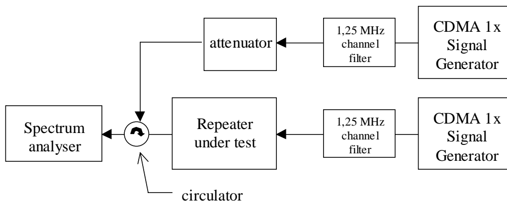
Figure D.6: Measuring system set-up for output intermodulation
