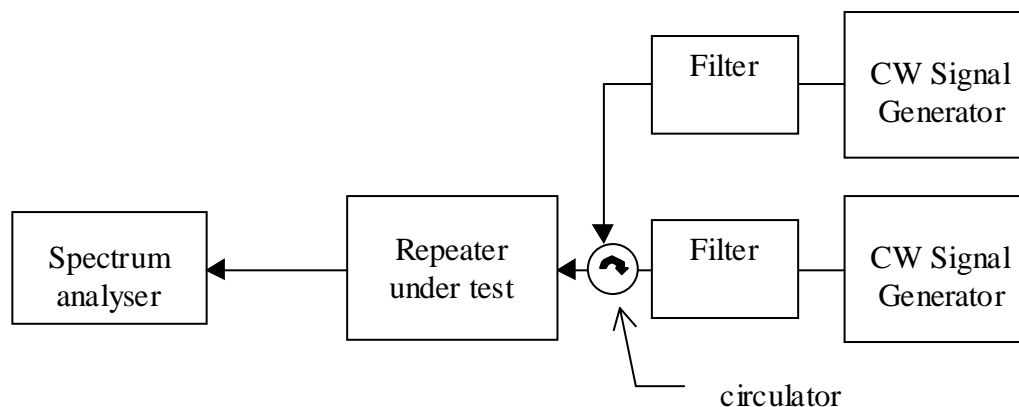
Figure D.3: Measuring system set-up for input intermodulation
