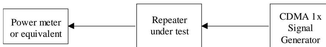
Figure D.5: Measuring system set-up for Adjacent Channel Rejection Ratio (ACRR)
