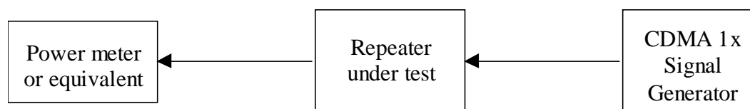
Figure D.2: Measuring system set-up for maximum output power
