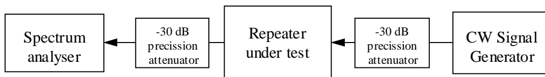
Figure D.4: Measuring system set-up for out of band gain
