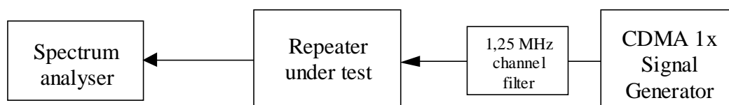
Figure D.1: Measuring system set-up for transmitter conducted unwanted emission
