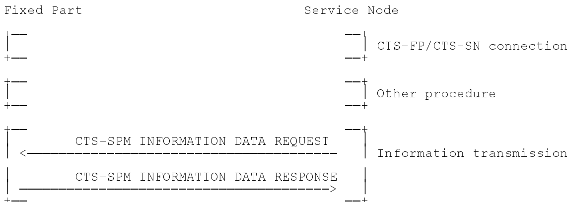
Figure 5.4/GSM 04.xx: Information request procedure
