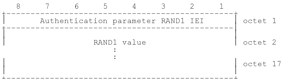
Figure 10.x/GSM 04.xx Authentication Parameter RAND1 information element
