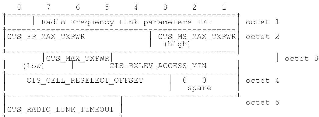
Figure 10.2/GSM 04.xx Radio Link Control Parameters information element
