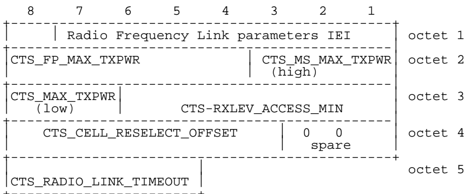
Figure 10.2/GSM 04.xx Radio Link Control Parameters information element
