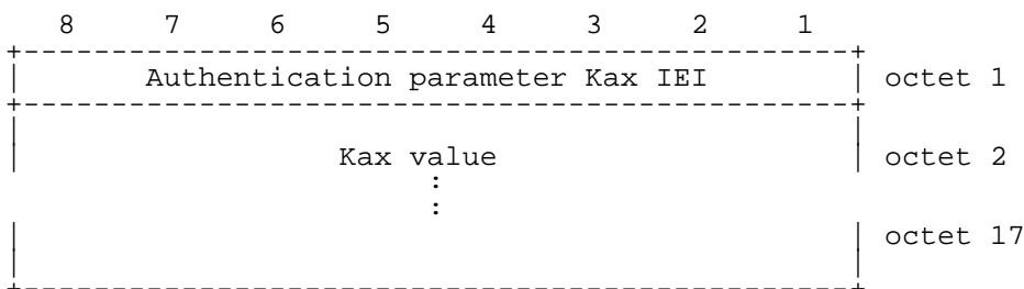
Figure 10.16/GSM 04.56 Authentication Parameter Kax information element
