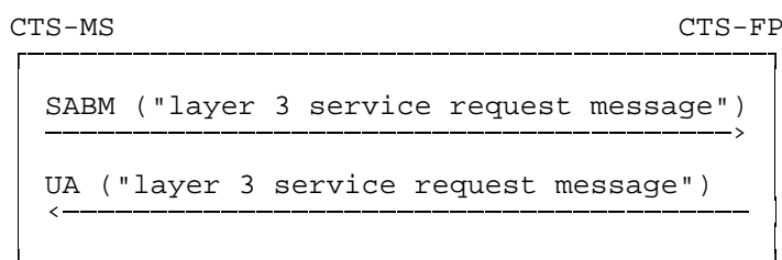
Figure 4.1/GSM 04.56 Service request and contention resolution
