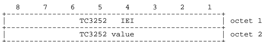
Figure 10.21/GSM 04.56 TC3252 information element
