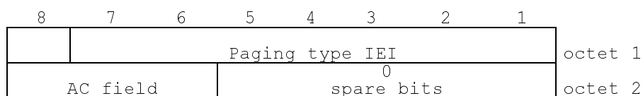
Figure 10.1/GSM 04.56 Paging type information element
